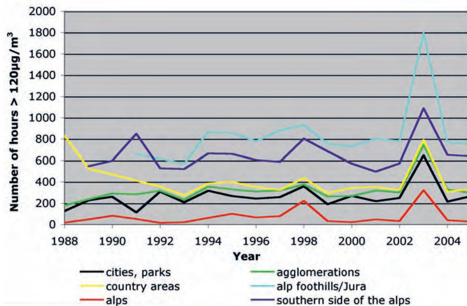
Figure 3: Number of hours per year with ozone concentrations over 120 µg/m³ at NABEL measuring stations in cities/parks (black), agglomerations (green), country areas (yellow), Alp foothills/Jura (blue), Alps (red) and the southern side of the Alps (purple). (Source: NABEL, BAFU and Empa)
