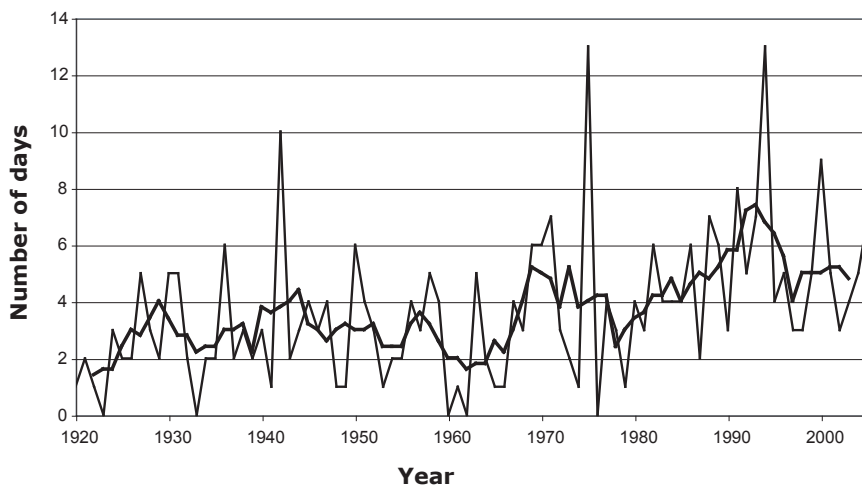
Figure 5: Time series of the number of hail days with 100 or more affected municipalities from 1920–2005. The increasing trend of intense hail days between 1980 and 1994 is clearly visible. (Source: Hans-Heinrich Schiesser)
