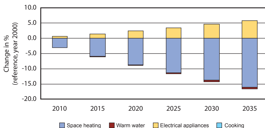
Figure 4: Changes in energy consumption in private households according to type of use, compared to the reference scenario (today: 75,000 GWh) 5 .
